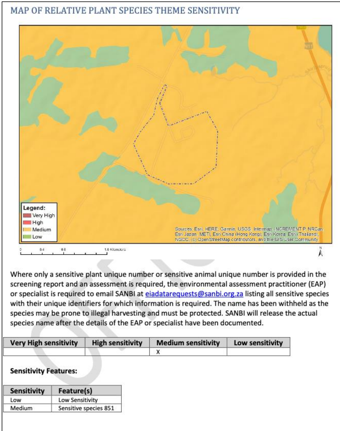
Figure 5-9: Relative Plant species sensitivity Sivutse A and B
