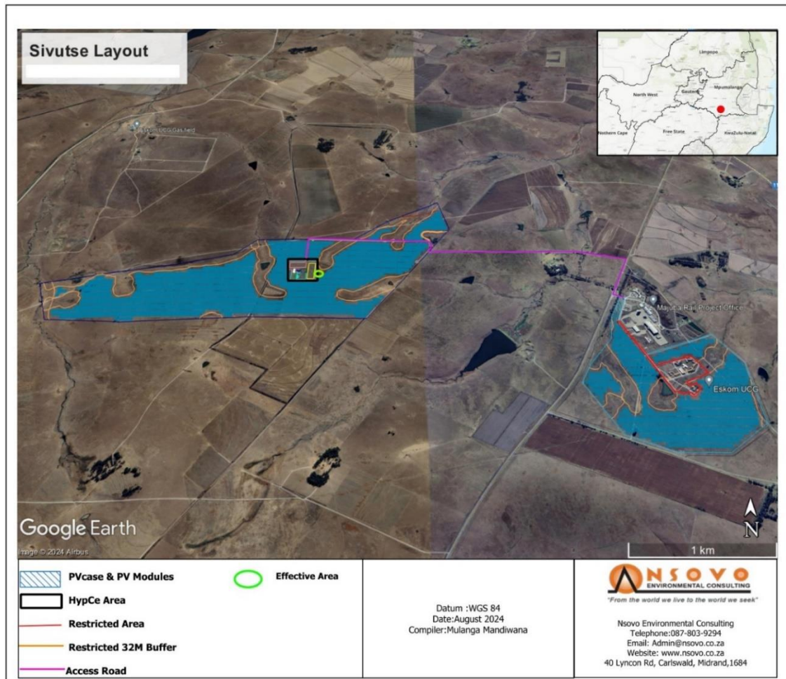
Figure 1-2: Proposed infrastructure layout for Sivutse
