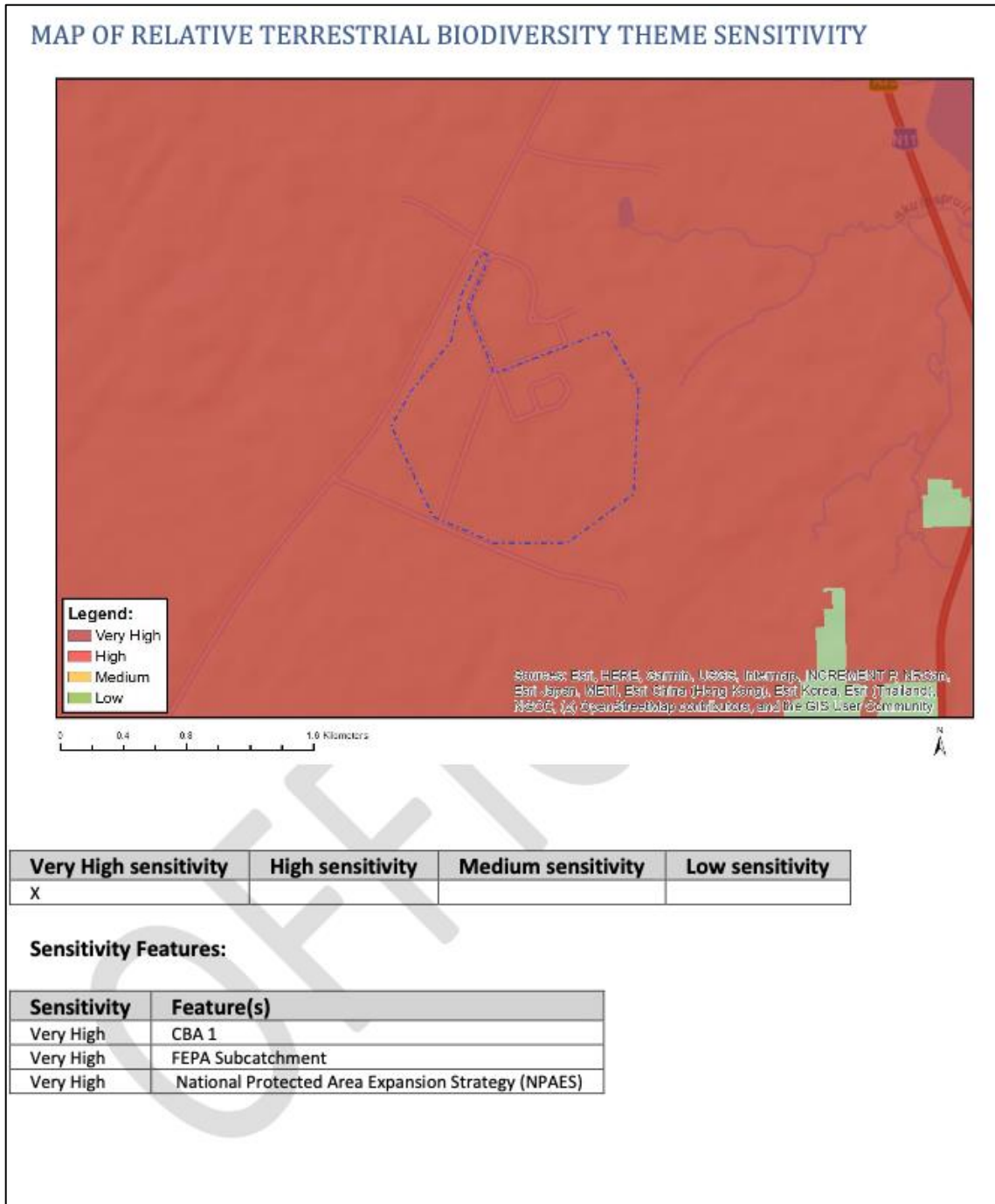
Figure 5-8: Relative Terrestrial Biodiversity Theme Sensitivity Sivutse A and B
