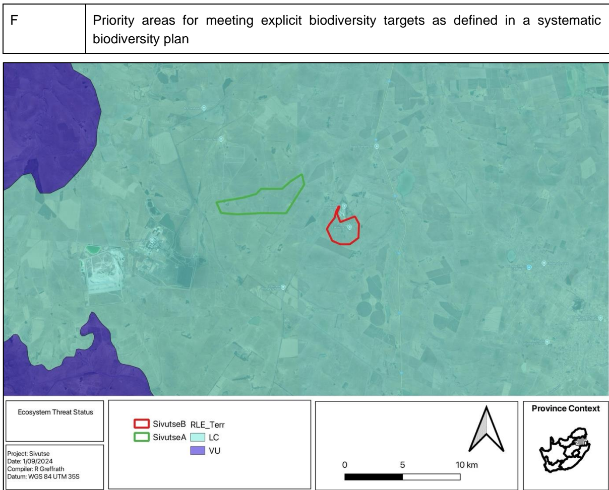
Figure 4-2: Ecosystem Threat Status
