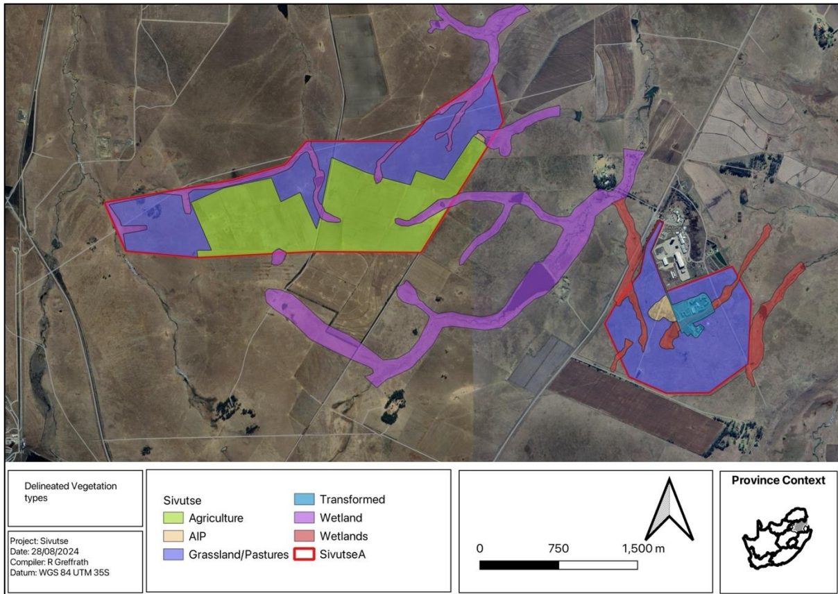
Figure 5-1: Delineated Vegetation types encountered within the Renewstable Sivutse project area.
